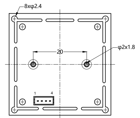
PH1.5,top entry type, 4 PINS
